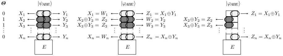
Fig. 1. Original and modified experiments for obtaining the same state \rho_{\theta W Z E_0} .
