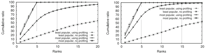
(a) 25% least and most popular domains (b) 5% least and most popular domains
