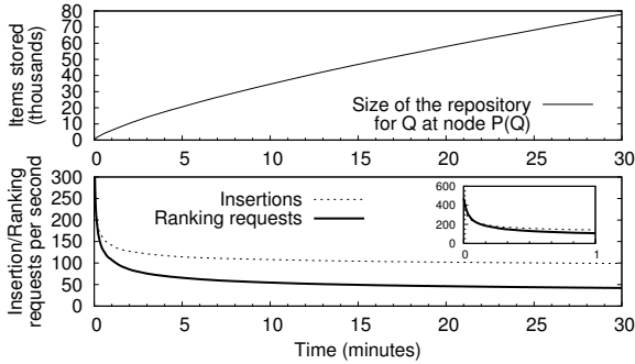
Fig. 5. Performance, single repository: max. possible load vs. repository size.
