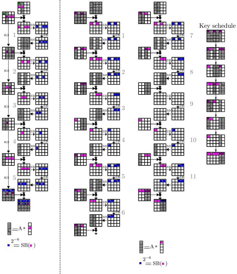
Fig. 2. The best characteristics for AES-128(left) and AES-192(right). The first one is on 5 rounds, while the second one is on 11 rounds.
