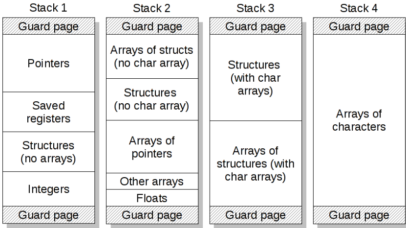
Fig. 1. Multistack stack layout for 4 stacks
