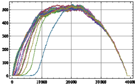
Fig. 3. An unstationar scenario with Forced-Friedman algorithm. The systems starts from the empty state and with constant rate of incoming peers, then after a while the flow of peers stops. The case with 50 chunks, populations of nodes having particular chunks. The system manages to complete, all peers complete without any long tail of delay.
