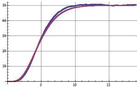
Fig. 7. A simulation for 20 chunk-system with Forced-Friedman algorithm, \lambda = 50 . A bit rugged line is simulated processes for n_5 , empirical average over 1000 experiments, the smooth line is solution of the differential equations for the simplified model. It seems, that the average of the steady state is converging to the one for the simplified process. However, the transient state is slightly deviating from it, possibly having damping oscillations around the simplified system curve.
