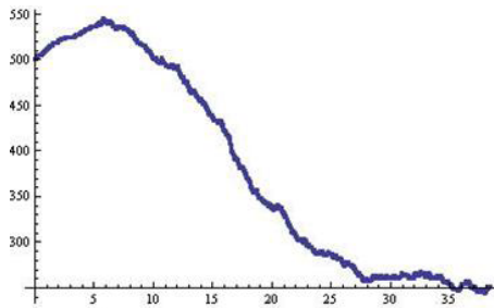
Fig. 4. Relaxation of the system with Forced-Friedman algorithm. The system starts from a state with 500 nodes missing the same chunk (a rare chunk), however, the system quickly relaxes to steady state. A case with 20 chunks, number of peers in the system is shown.
