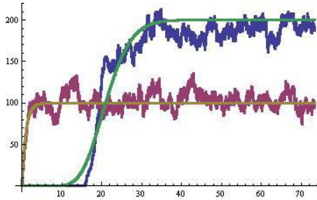
Fig. 6. A simulation for 20 chunk-system with Forced-Friedman algorithm, \lambda = 100 . The rugged lines are simulated processes for n_1 and n_{19} , while the smooth lines are solutions of the differential equations for the simplified model. Other components have similar behavior.
