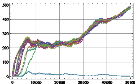
Fig. 1. A result of a computer simulation with a simple random contact system, without favoring rare chunks. Each line represents the size of a particular chunk population, number of nodes in the system with given chunk, for system starting from a system with one ‘seed’ as a function of time (a sample path). Number of chunks m = 20 and \lambda = 10 times the contact rate. The populations of nodes that have certain chunks blows up, except for one chunk that remains ‘rare’.
