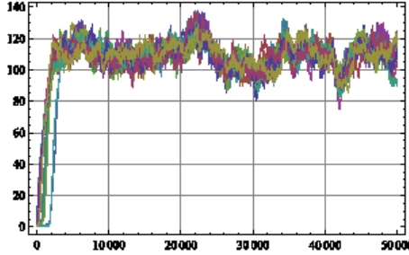
Fig. 2. A computer experiment with random contact system with Forced-Friedman random contacts, m = 20 , \lambda = 100 . The sizes of chunk populations are shown starting from system with only the seed node. A good balance seem to prevail and a good performance, since no accumulation of peers is not seen although there is a constant flow of incoming peers into the system.
