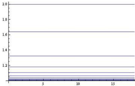
Fig. 5. Levels of steady state population sizes of nodes with 1, 2, \dots , m - 1 chunks in units of \lambda , the accumulation point of lines equals to 1.
