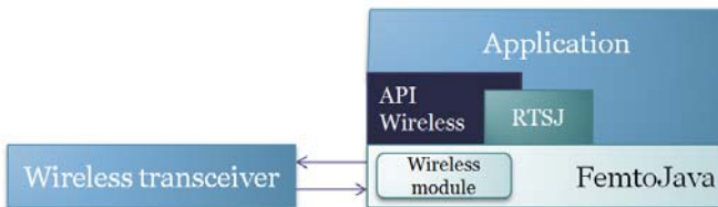
Fig. 2. FemtoNode Architecture with API-Wireless
