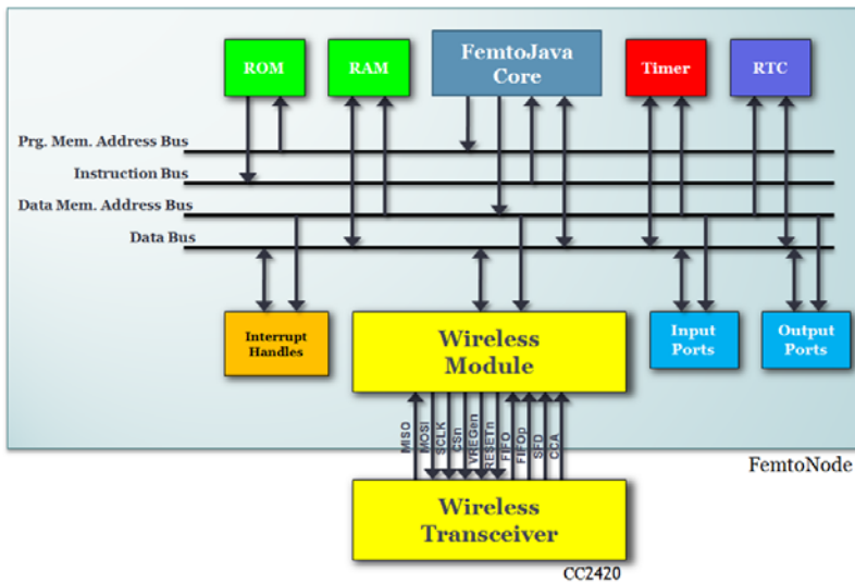
Fig. 1. Hardware Architecture of FemtoNode
