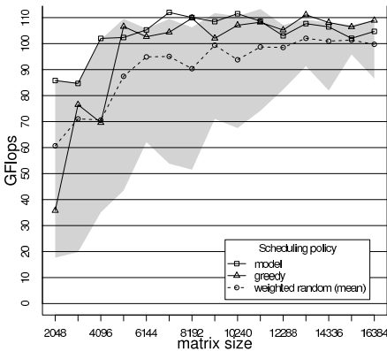
Fig. 3. Blocked Matrix Multiplication
