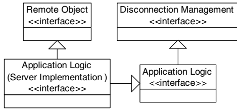
Fig. 1. Hierarchy of interfaces for disconnection-aware components
