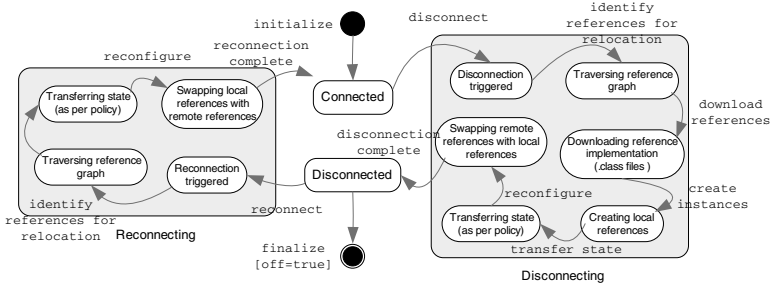
Fig. 2. State-transition diagram from disconnection/reconnection management
