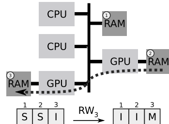
Fig. 2. Coherence protocol
