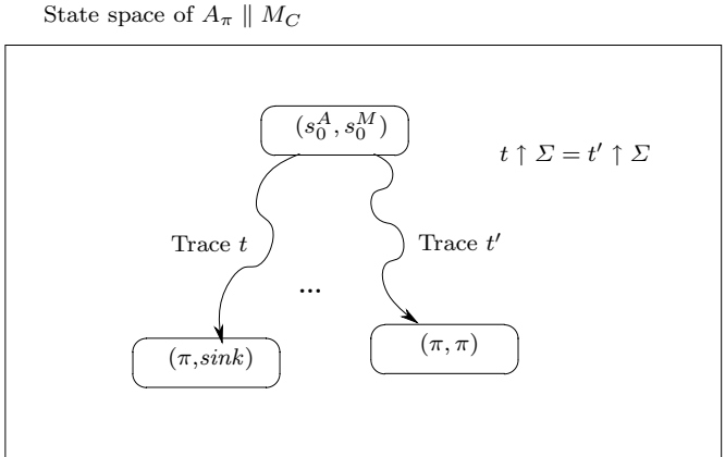
Fig. 3. Example for Oracle 2: dealing with non-determinism
