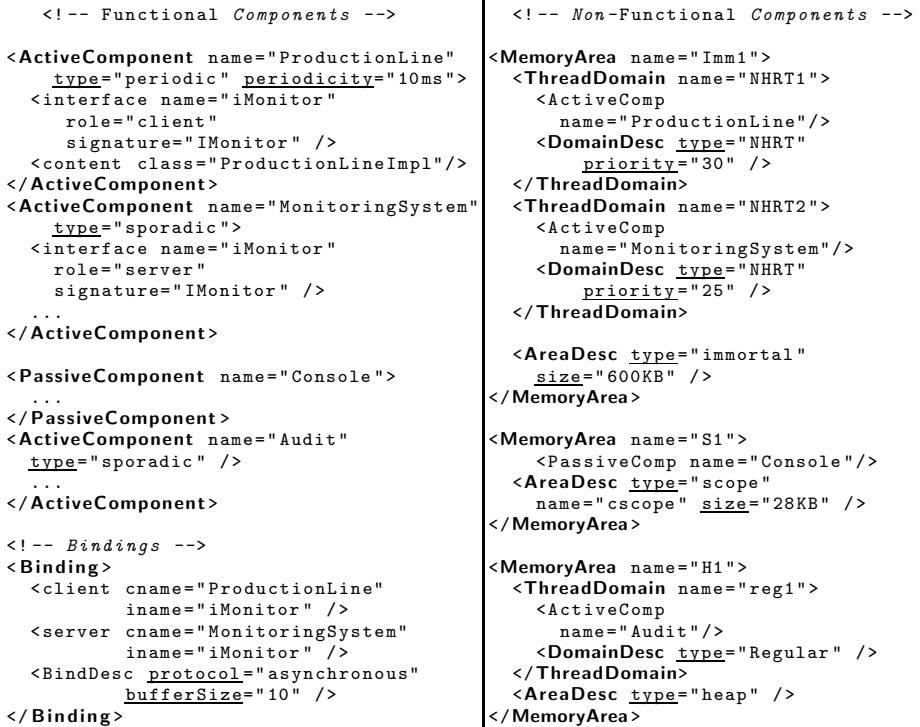
Fig. 4. Motivation Example: Real-time System Architecture
