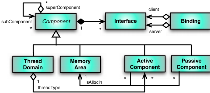
Fig. 2. A Real-Time Component Metamodel
