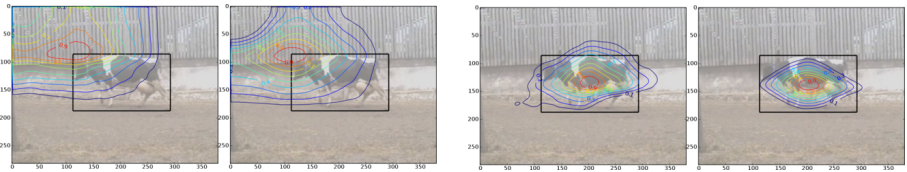
Fig. 4. Contour plots of the learned quality function for a TU Darmstadt cow test image (best viewed in color). The first and third image corresponds to the quality function learned by binary training, the second and fourth image shows structured training. In left block shows the quality of the upper left corner when fixing the bottom right corner at its ground truth coordinates. The right block shows the quality of the center point when keeping the box dimensions fixed at their ground truth values. Structured learning achieves tighter contours, indicating less uncertainty in localization.
