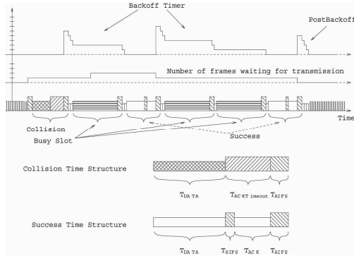
Fig. 1. AC channel access time-sequence
