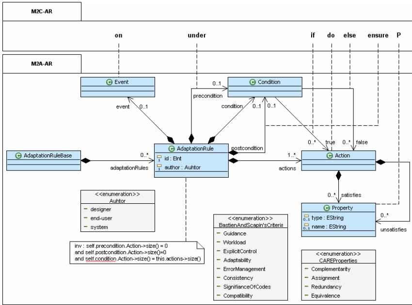
Fig. 5. Our meta-model for adaptation rules
