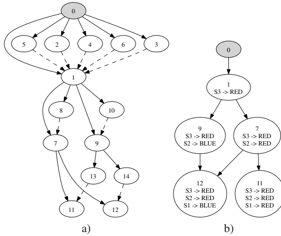
Fig. 6. State space of the Triangle example from Fig. 1, where exploration of isomorphic states has been pruned. The dashed lines on (a) exhibit encounters of isomorphic states during exploration. (b) exhibits the structure of the state graph when isomorphic states are collapsed.
