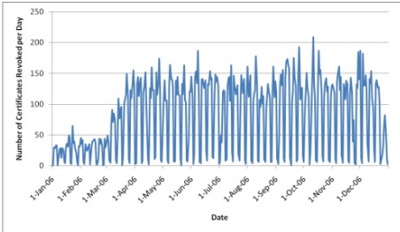
Fig. 7. Certificates Revoked Per Day (2006)
