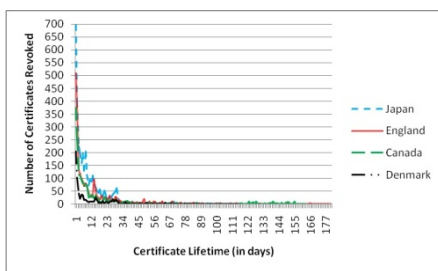
Fig. 5. Number of Certificates Revoked vs. Lifetime (Remaining Countries)
