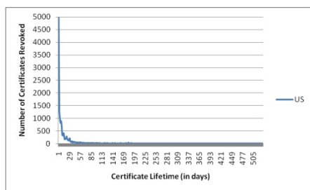
Fig. 4. Number of Certificates Revoked vs. Lifetime (United States)
