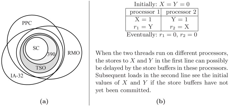
Fig. 1. (a) A comparison of various memory models [6,9,14,15,24]. (b) An execution that is possible on TSO but not on SC .
