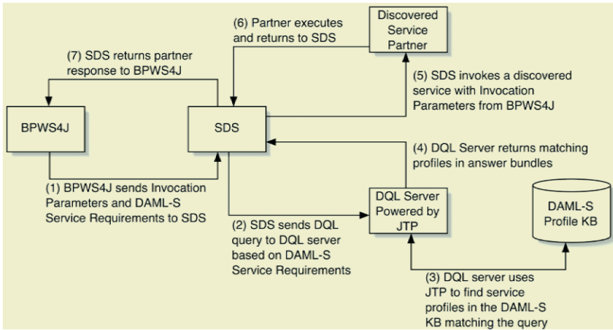
Fig. 2. Interaction flow between BPWS4J, SDS, DQL server, & discovered service partners.
