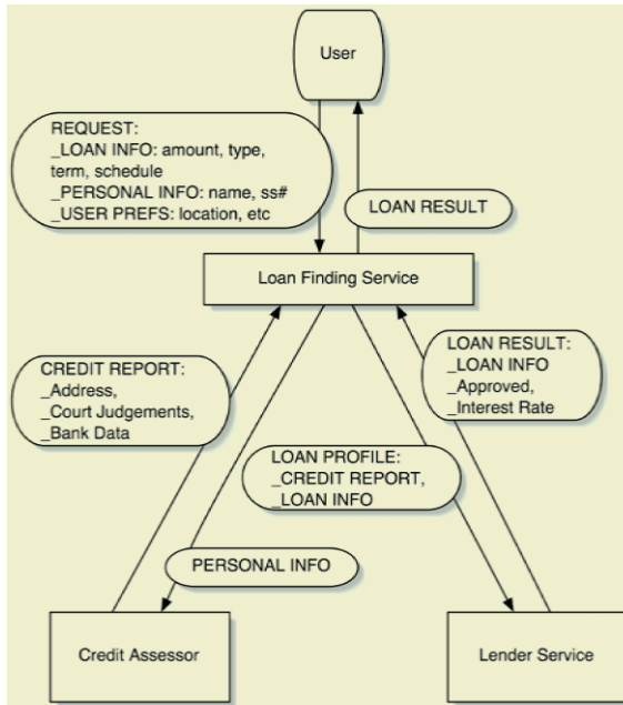
Fig. 1. An interaction model for the loan example domain.
