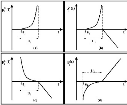
Fig. 1. a) Native UTL model b) c) d) Different stages leading to the hybrid queuing model.
