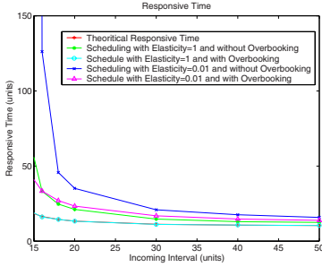
Fig. 1. Responsive Time (1 consumer vs. 1 supplier): \alpha_{consumer} = 1 , \alpha_{supplier} = 10 ; Ceiling_{consumer} = 7 , Floor_{supplier} = 4 ; \mu = 1/10
