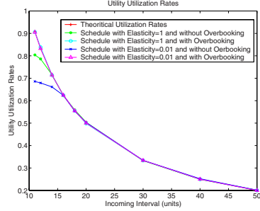
Fig. 2. Usage Rates (1 consumer vs. 1 supplier): \alpha_{consumer} = 1 , \alpha_{supplier} = 10 ; Ceiling_{consumer} = 7 , Floor_{supplier} = 4 ; \mu = 1/10
