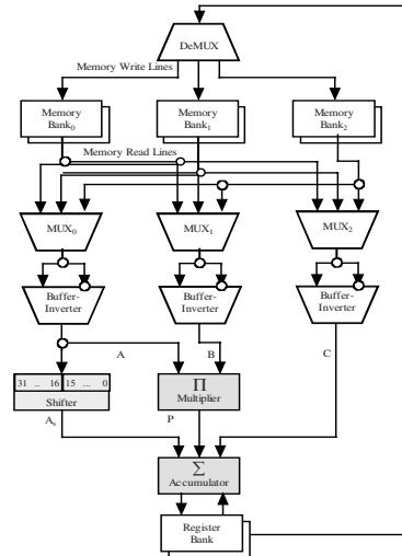
Fig. 1. Dataflow diagram
