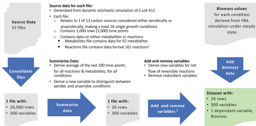
Fig. 1. Summary of data preparation steps. A dataset was created for analysis with 300 variables and 26 single growth conditions, later extended by 156 pairwise conditions.
