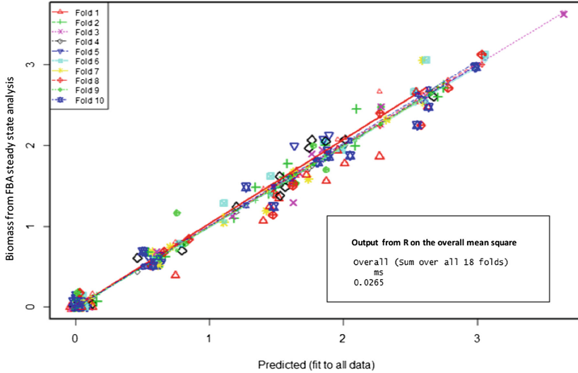
Fig. 5. Cross-validation output for the final regression model. Small symbols show predicted values; large symbols represent actuals. The 10 dashed lines relate to the best fit line for the respective folds.
