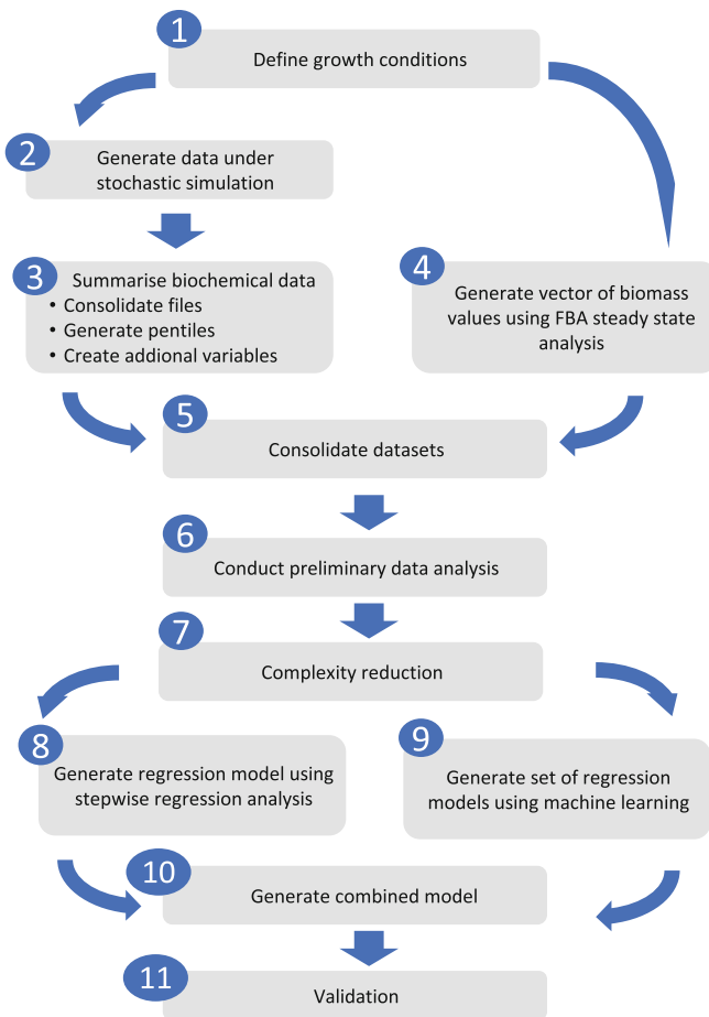
Fig. 2. Workflow of key analytical steps in the development of the proxy function. Steps 1–5 are covered in Sect. 3, steps 6–10 in Sect. 4 and step 11 in Sect. 5.
