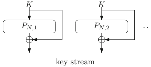
Fig. 4. Encryption mode of Rasta.
