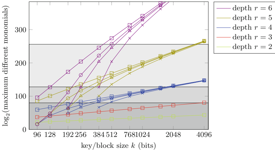
Fig. 5. Trivial linearization attack. \square/\circ/\Delta/\times denote 0/80/128/256-bit key guess.
