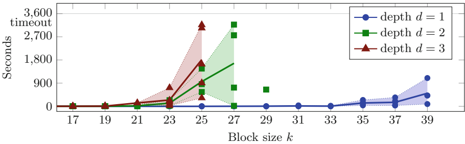
Fig. 8. SAT solver runtime for successful key-recovery on toy parameter sizes: Average, minimum, and maximum runtime for up to 8 challenges per block size.
