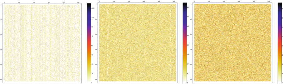
Fig. 9. Pollock representation of the LAT for 1, 2 and 3-round versions of one instance of the cipher on 9 bits.
