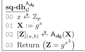
Fig. 3. Algebraic adversary \mathcal{A}_{\text{alg}} playing in \mathbf{sq-dh}_G .
