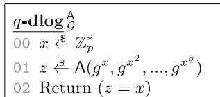
Fig. 13. q -Discrete Logarithm Game q - dlog relative to \mathcal{G} and adversary A .
