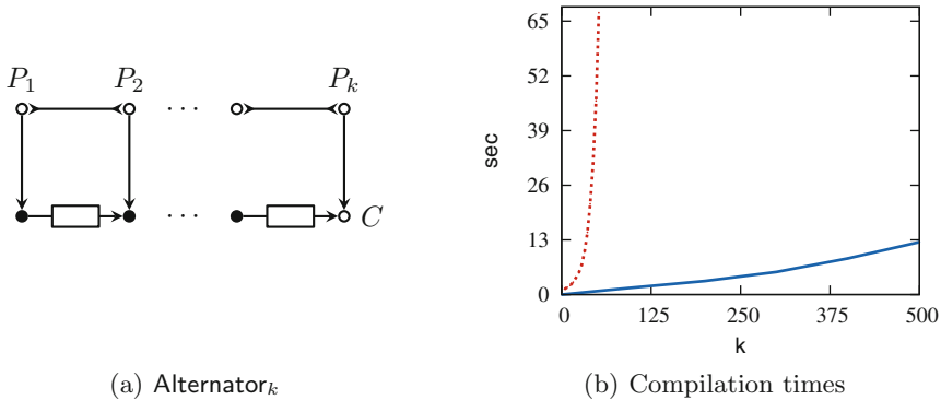
Fig. 3. Graphical representation (a) of the Alternator k protocol in [17], for 2 \leq k \leq 500 , and its compilation time (b). The dotted red line is produced by the Jongmans' compiler (and corresponds to [17, Fig.11(a)]), and the solid blue line is our compiler. (Color figure online)
