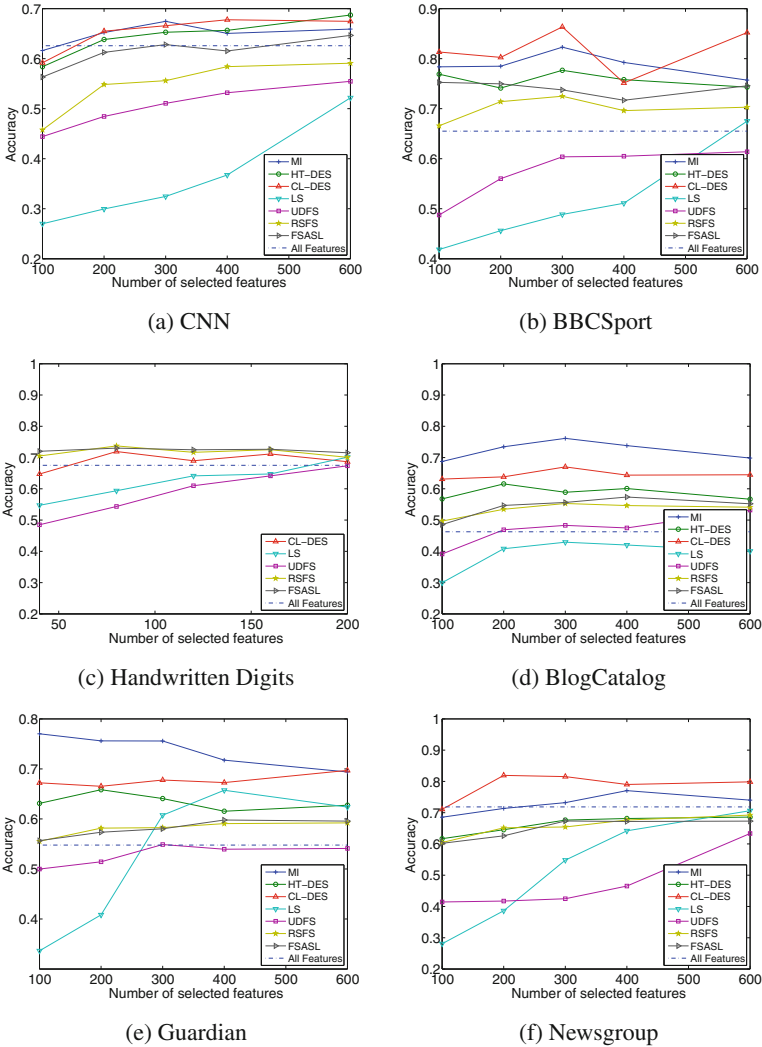
Fig. 2. Accuracy of clustering results
