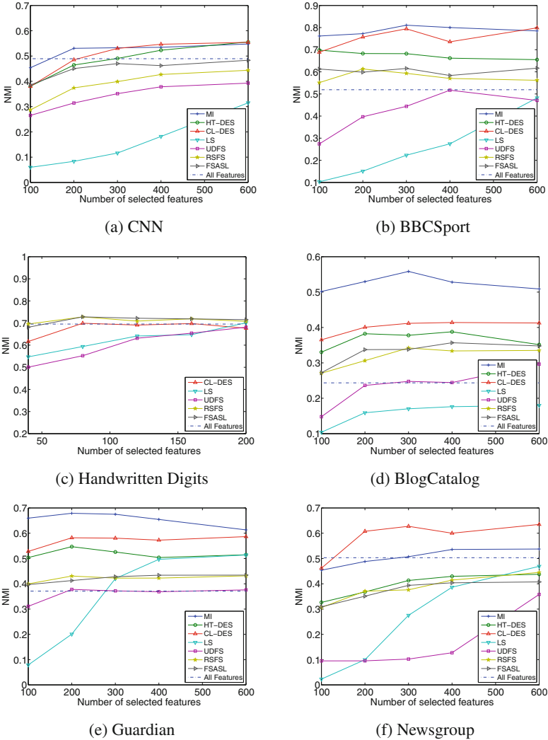
Fig. 3. NMI of clustering results
