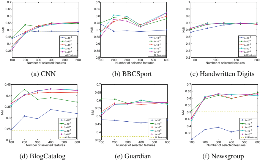
Fig. 4. NMI of clustering results with features selected by CL-DES under different values of \lambda
