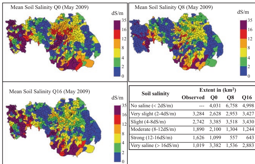
Fig. 28.14 \Delta DIEM soil salinity results for May 2009 (Source of observed area, SRDI (2012))
