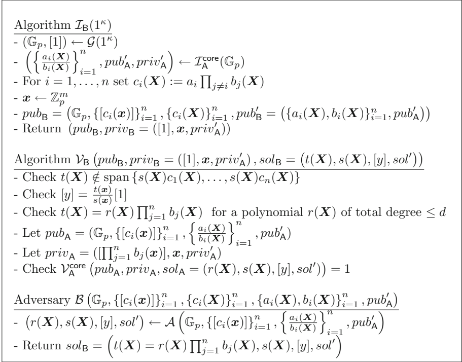
Fig. 3. Simple target assumption B = (\mathcal{I}_B, \mathcal{V}_B) and adversary \mathcal{B} against it
