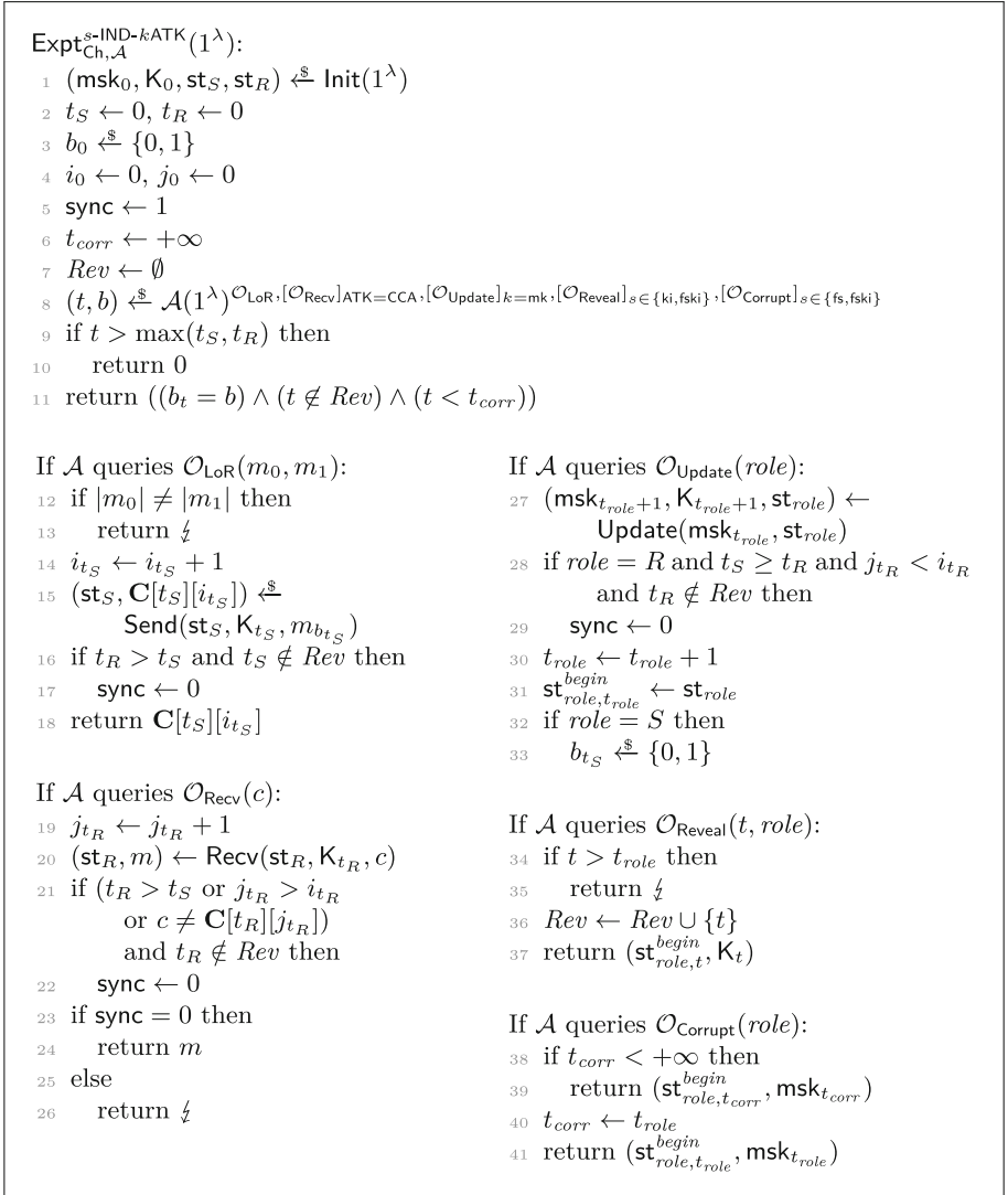
Fig. 2. Security experiment for confidentiality (sIND-kATK) of a multi-key channel Ch. An adversary A has only access to an oracle [O X ] c if the condition c is satisfied.
