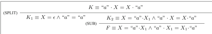
Fig. 2. Solving steps for Example 3
