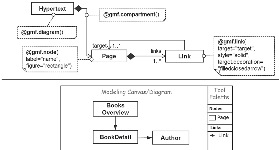
Fig. 1. GCS definition with EuGENia by-example.
