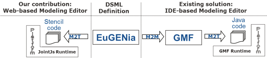
Fig. 2. Extending EuGENia with an additional M2T transformation to generate Stencils for JointJS.
