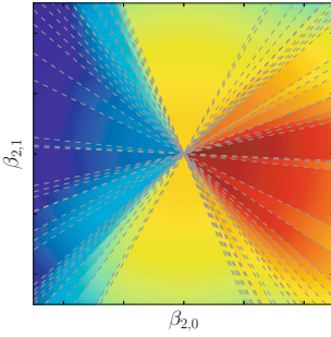
Fig. 2. A heatmap of the posterior distribution for a two-class toy problem with a 1D feature-space. Discontinuities are represented by gray stippled lines.
