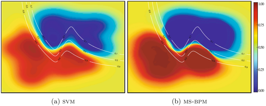
Fig. 4. Posterior class membership probabilities for the Ripley synthetic dataset. Both classifiers use an RBF kernel with \gamma = 7.5 as selected via grid search. The heatmaps show the posterior plots of the learned classification models while the overlaid contour plots depict the true probabilities. The MS-BPM classifier (right) tends to generate more confident predictions than the SVM classifier (left) and produces smoother class boundaries.
