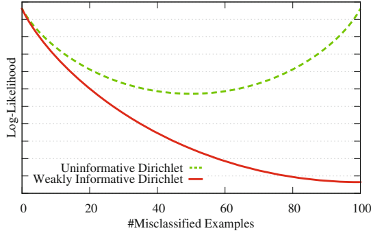
Fig. 1. Comparison of the log-likelihoods for a small training set ( N = 100 ) plotted over the number of misclassified examples. Models under comparison are the Dirichlet-multinomial model with an uninformative Dirichlet prior and a weakly informative Dirichlet prior.
