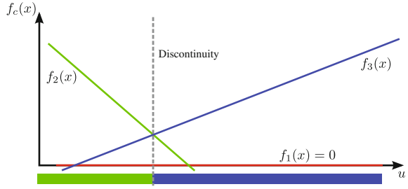
Fig. 3. Example of a three-class problem. The upper envelope of the linear predictor functions defines the partition membership intervals for one individual training example \mathbf{x} along the search path. In this particular case, class 2 is selected left of the discontinuity and class 3 otherwise. Class 1 is never selected.
