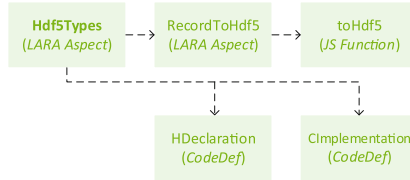
Fig. 5. use relationships for the aspect Hdf5Types .
