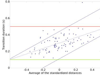
Fig. 8. More than 90% of the values is contained in the area bounded by the lines.
