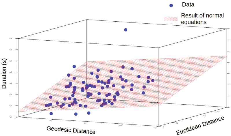
Fig. 11. Surface computed using normal Eq. (4) with the manual annotation data.
