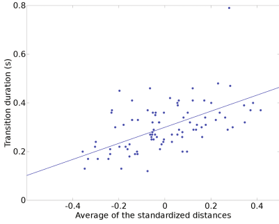
Fig. 7. Duration of the transitions in function of the average of the two normalized distances.
