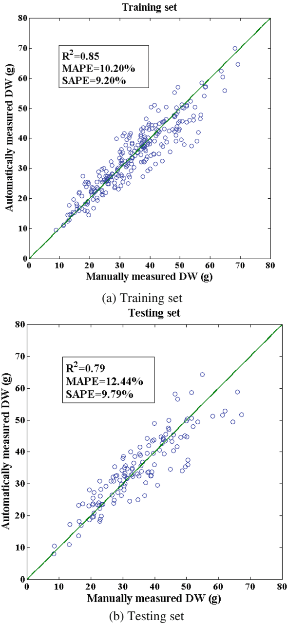
Fig. 2. Performance of the final DW model (ASR-GA-SVR model)
