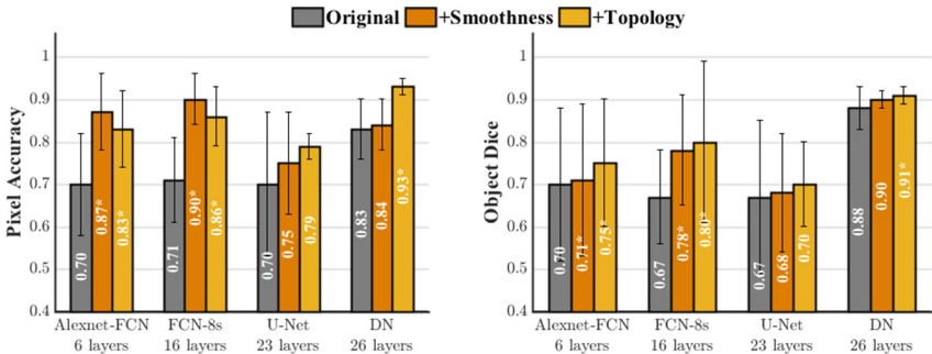
Fig. 2. Advantage of the proposed loss: “Origina” refers to the cross-entropy loss \mathcal{L} . “+Smoothness” refers to using the proposed penalty term \mathcal{L}_S and “+Topology” refers to adding our topology prior \mathcal{L}_T . The asterisk (*) corresponds to statistically significant differences from the original models obtained using a Wilcoxon matched-pairs signed rank sum test at p < 0.05 .
