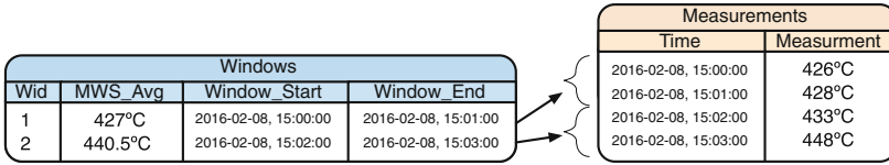
Fig. 2. Schema for storing archived streams and MWSs
