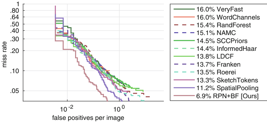
Fig. 7. Comparisons on the INRIA dataset (legends indicate MR).
