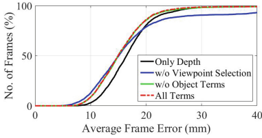
Fig. 6. Ablative analysis
