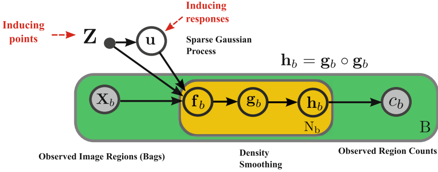
Fig. 2. Plate diagram of the proposed model. For simplicity, the diagram pretends that the annotated regions do not overlap, B_b \cap B_{b'} = \emptyset for b \neq b' . Our actual model is not limited by this assumption.
