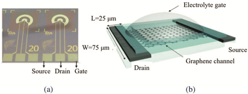
Fig. 1. (a) Photograph of two EGFETs on a silicon wafer, (b) schematic diagram showing the drain and source dimensions.
