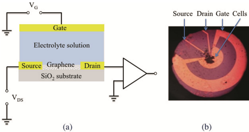
Fig. 2. (a) Schematic diagram showing the electrical connections to the EGFET. Low noise amplifiers were used to record the signals in current as well as in voltage, (b) Photograph showing a cluster of cardiomyocytes on top of the gate terminal.
