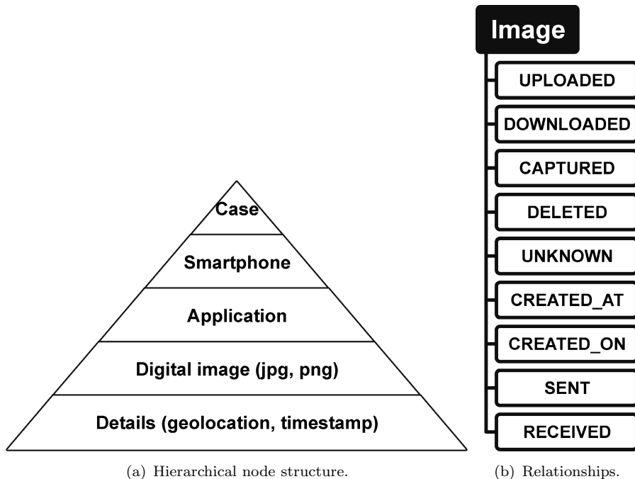
Figure 2. Graph database conceptual design.
