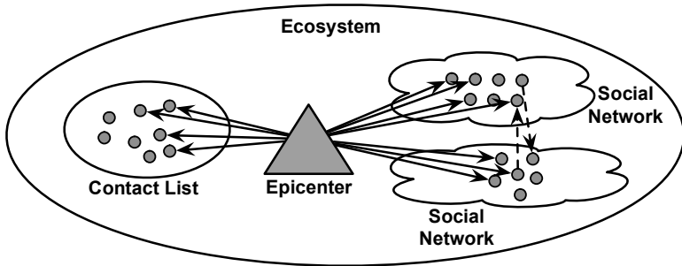
Figure 1. Smartphone ecosystem.
