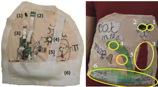
Fig. 5. Wearable hardware (1) push button; (2) camera; (3) Raspberry Pi B and Wi-Fi; (4) GPS; (5) LEDs for feedback; (6) battery pouch with two 1500 mAh batteries (GPS and Wi-Fi) and a USB charger (Raspberry Pi).
