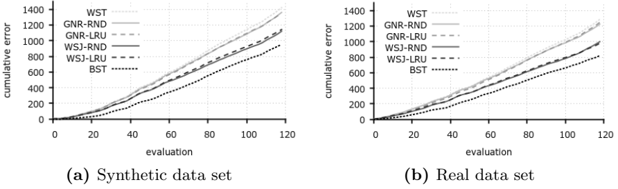
Fig. 3. Evaluation of the WSJ proposer
