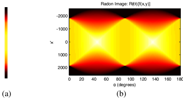
Fig. 4. Radon image obtained from the waterfall diagram of HSFV: (a) without magnification, and (b) with magnification
