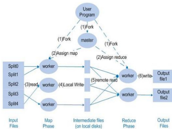
Fig. 1. MapReduce operation
