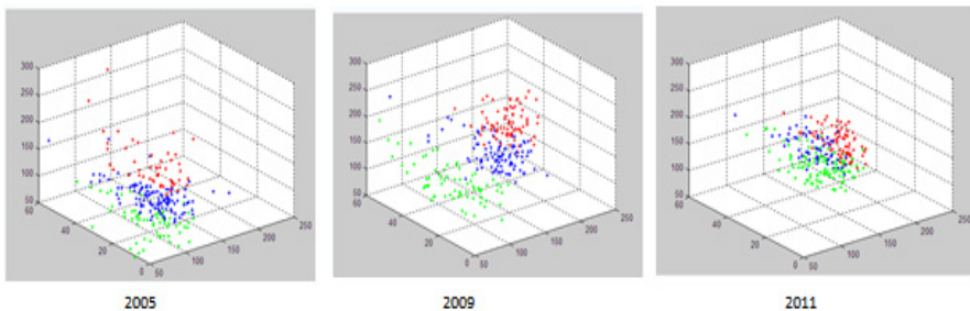
Fig. 3. Clustering results
