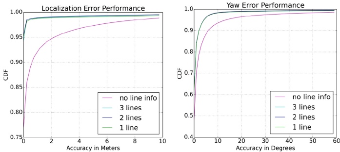
Fig. 1. CDF of localization error (left) and yaw error (right) for using K = 1, 2, 3 when incorporating line information. For comparison, not using line information (purple line) is shown as well (Color figure online).
