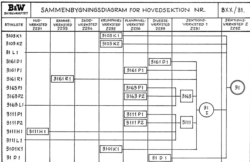
Fig. 5. Assembly chart
