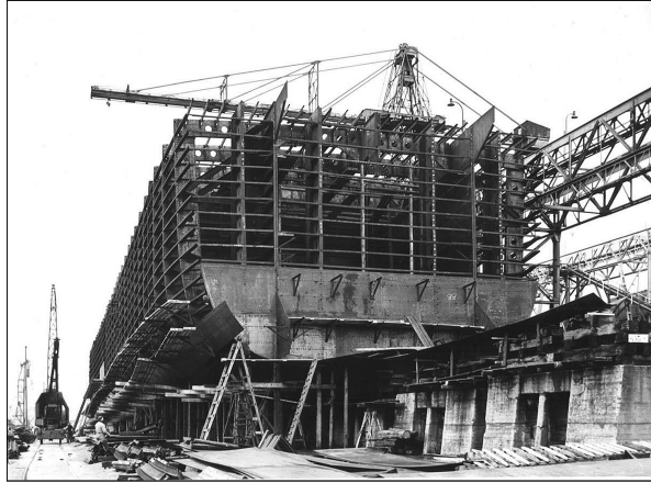
Fig. 2. Building berth on old shipyard
