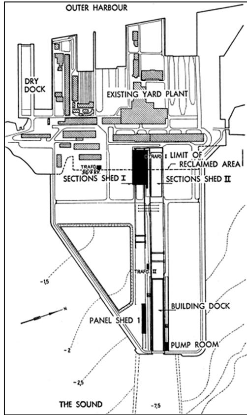
Fig. 3. Layout of new shipyard concept
