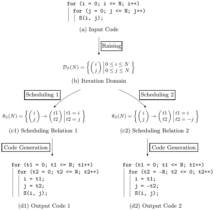
Fig. 1. Polyhedral Transformation Workflow For Two Example Versions
