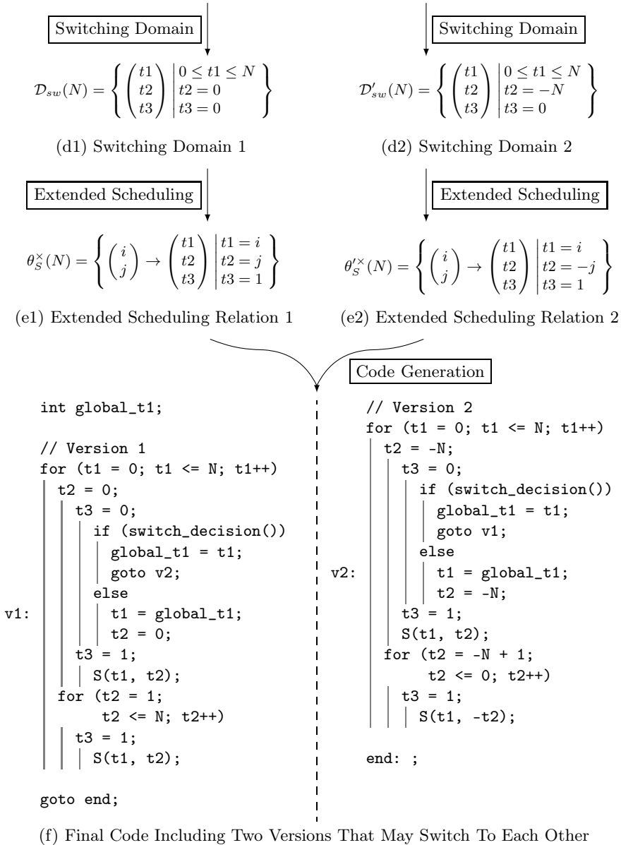
Fig. 2. (Our Alternative End of Fig. 1) Generation of a Multi-Version Code
