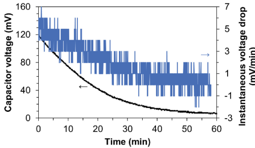
Fig. 6. Dependence of measured capacitor voltage and calculated instantaneous voltage drop on time for a 100 μF capacitor connected in the cough sensing system.
