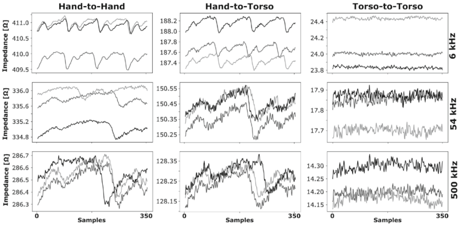
Fig. 2. Synchronized raw signals from one subject during one session. The columns represent the different electrode locations, and the rows represent the used frequencies.
